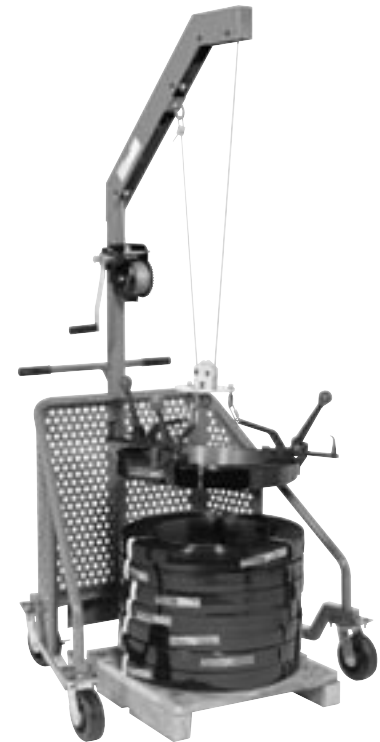
DF-10RW Accepts mill wound or ribbon wound coils 3/4" and 1-1/4" in width.
