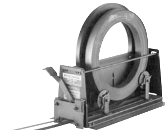
DC-1A Built-in strap cutter for pre-cutting. Holds any two ribbon wound coils.
